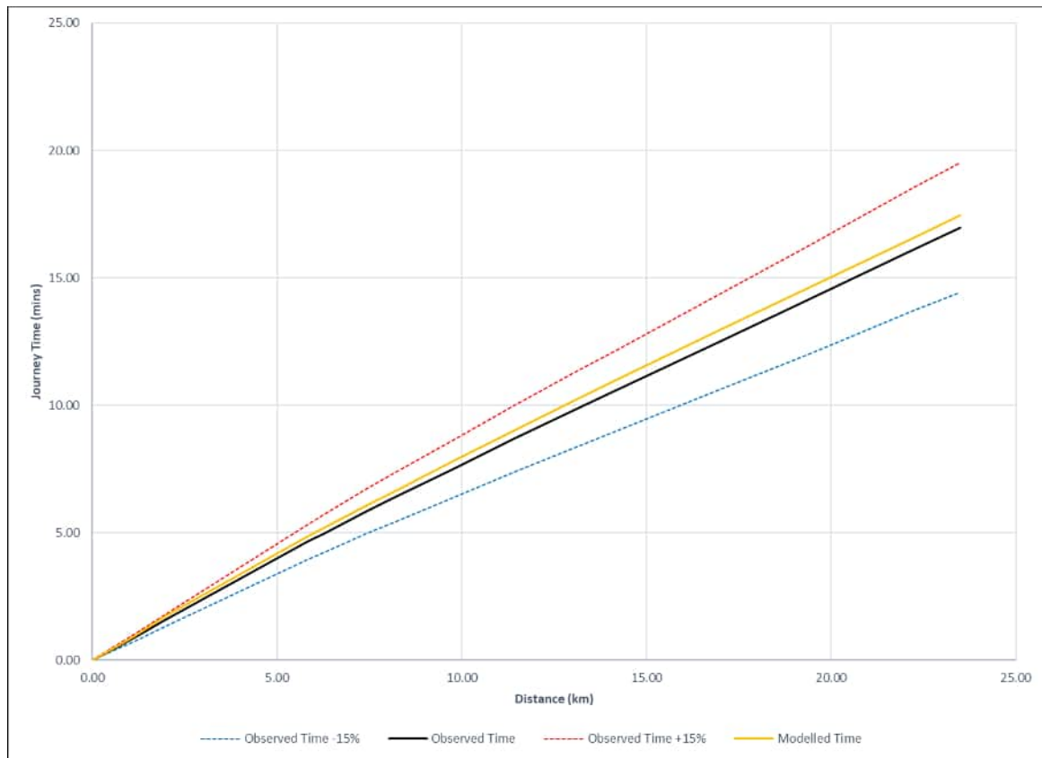
Plate E.155 Route 201 – M25 junction 30 – M2 junction 1 (inter-peak HGV)
