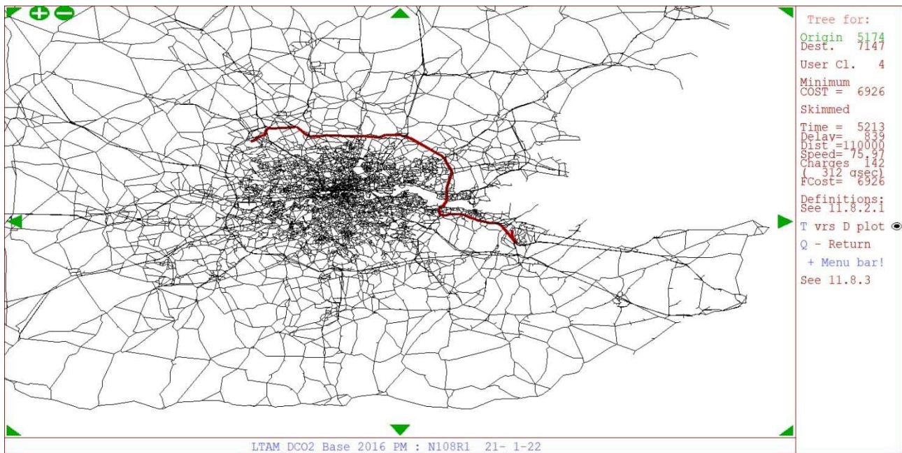
Plate B.66 Origin zone 5174 (Rickmansworth) to destination zone 7147 (Rochester) – (PM peak car commute high income)
