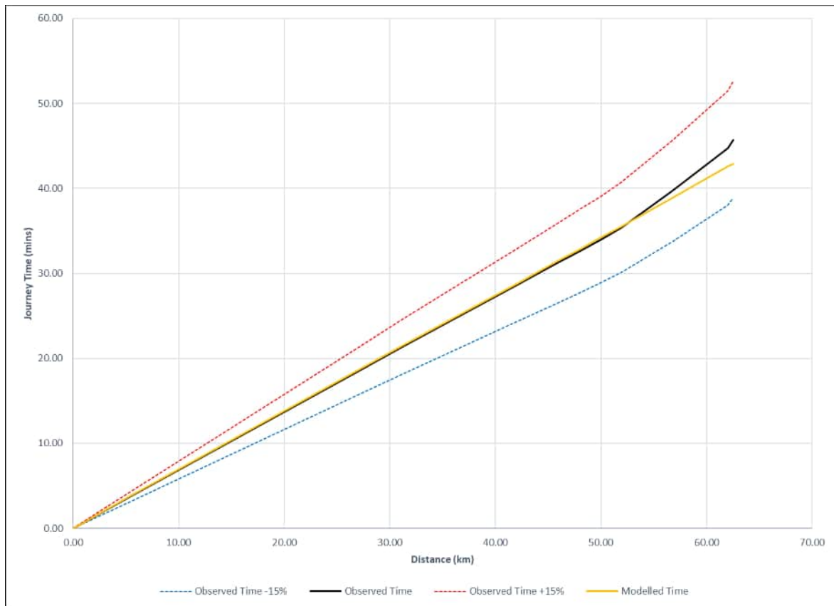
Plate E.59 Route 123 – M20/A20 junction 7 – Dover EB (AM peak HGV)
