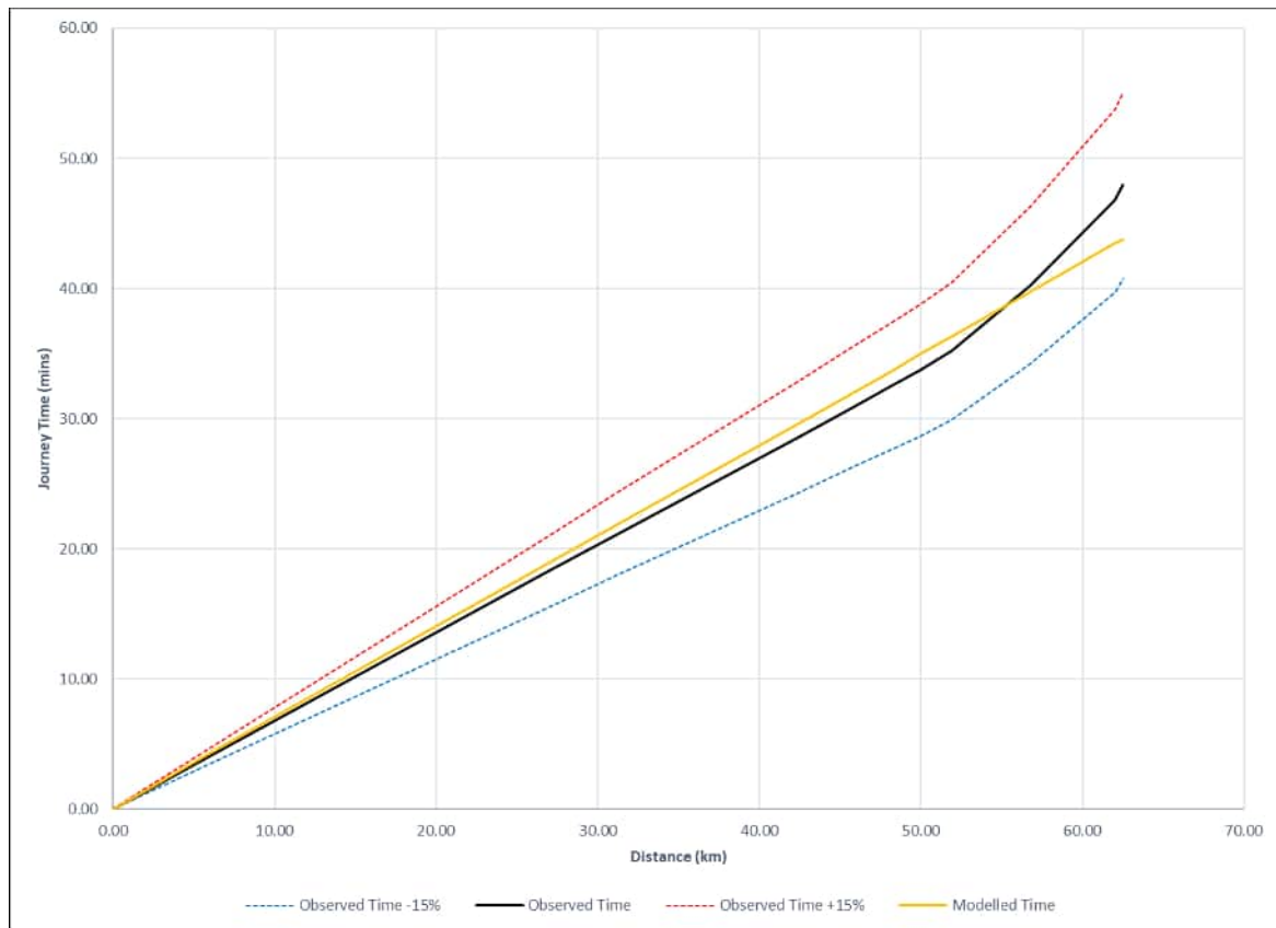
Plate E.215 Route 123 – M20/A20 junction 7 – Dover EB (PM peak HGV)
