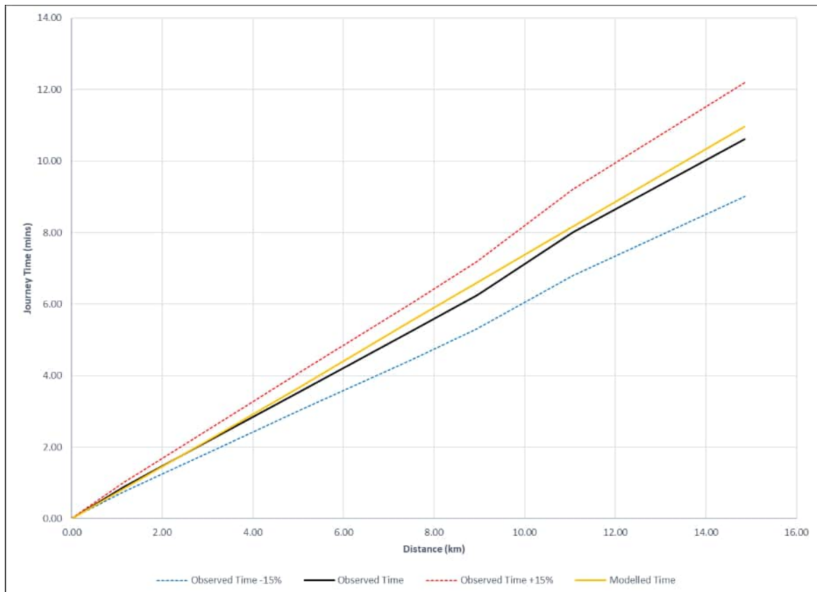
Plate E.128 Route 114 – A2 M2 junction 1 – M25 junction WB (inter-peak HGV)
