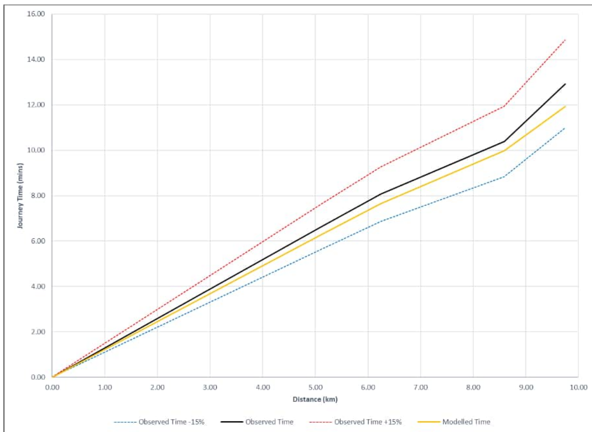
Plate E.74 Route 154 – A228 M2 junction – M20 junction SB (AM peak HGV)
