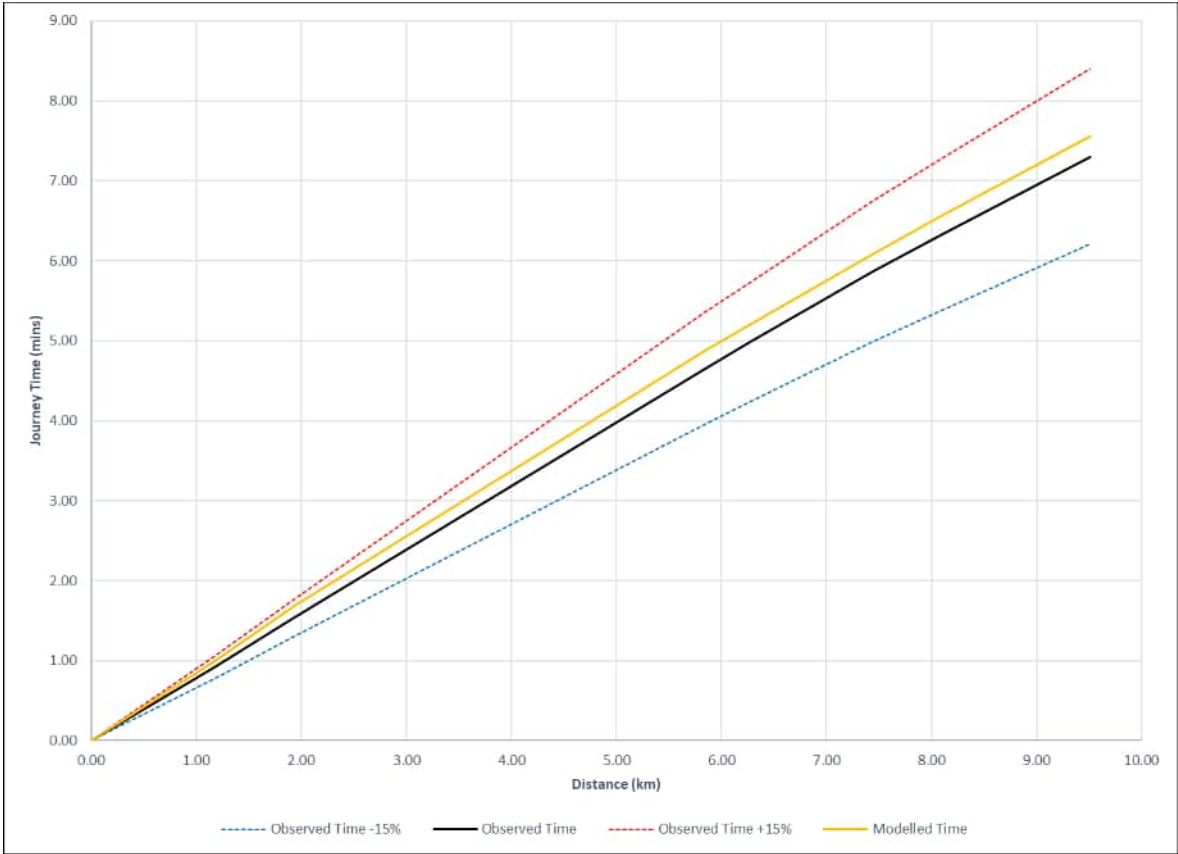
Plate E.120 Route 103 - M25 J30 - J2 CW (A282) (Inter Peak HGV)
