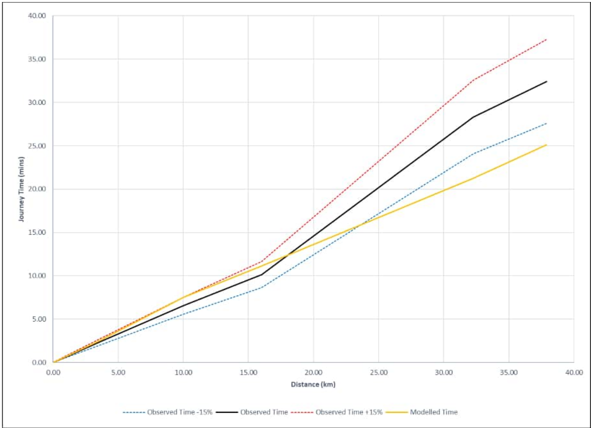
Plate E.6 Route 105 –east tunnel M 25 junction 2 – east tunnel junction 7 CW (AM peak lights)
