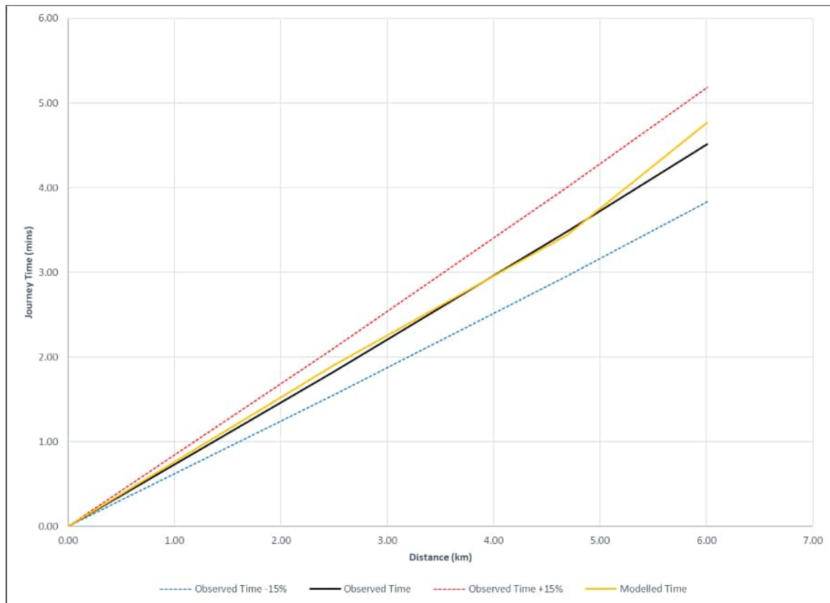
Plate E.192 Route 157 – A229 M20 junction – M2 junction NB (PM peak Lights)
