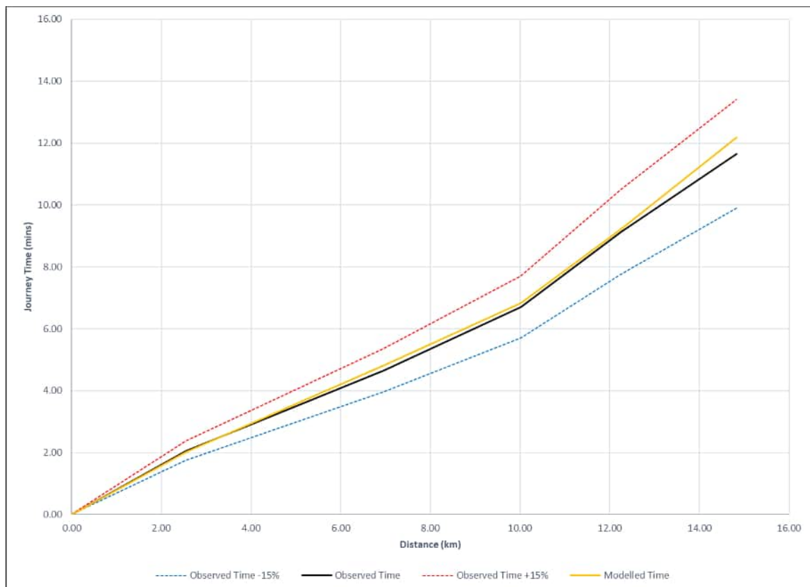
Plate E.179 Route 126 – A13 M25 junction – North Circular WB (PM peak Lights)
