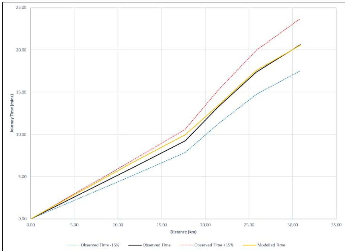
Plate E.174 Route 121 – M20 junction 1 – junction 7 EB (PM peak Lights)
