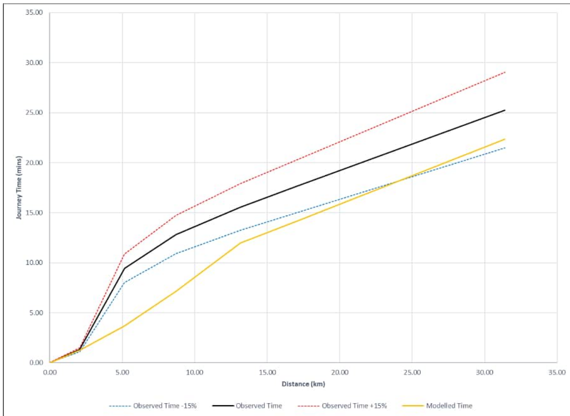
Plate E.19 Route 122 – M20 junction 7 – junction 1 WB (AM peak lights)
