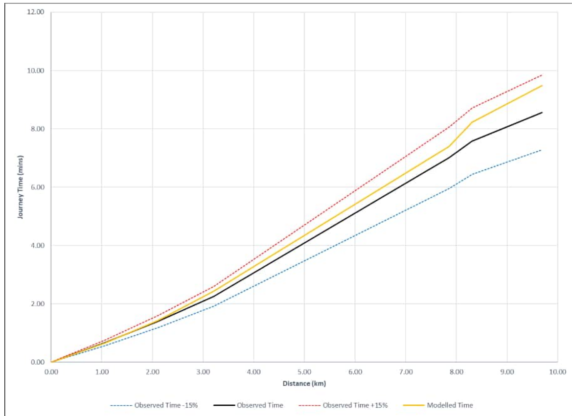
Plate E.5 Route 104E – M25 junction 2 – junction 30 ACW (A282) via East Tunnel (AM peak lights)
