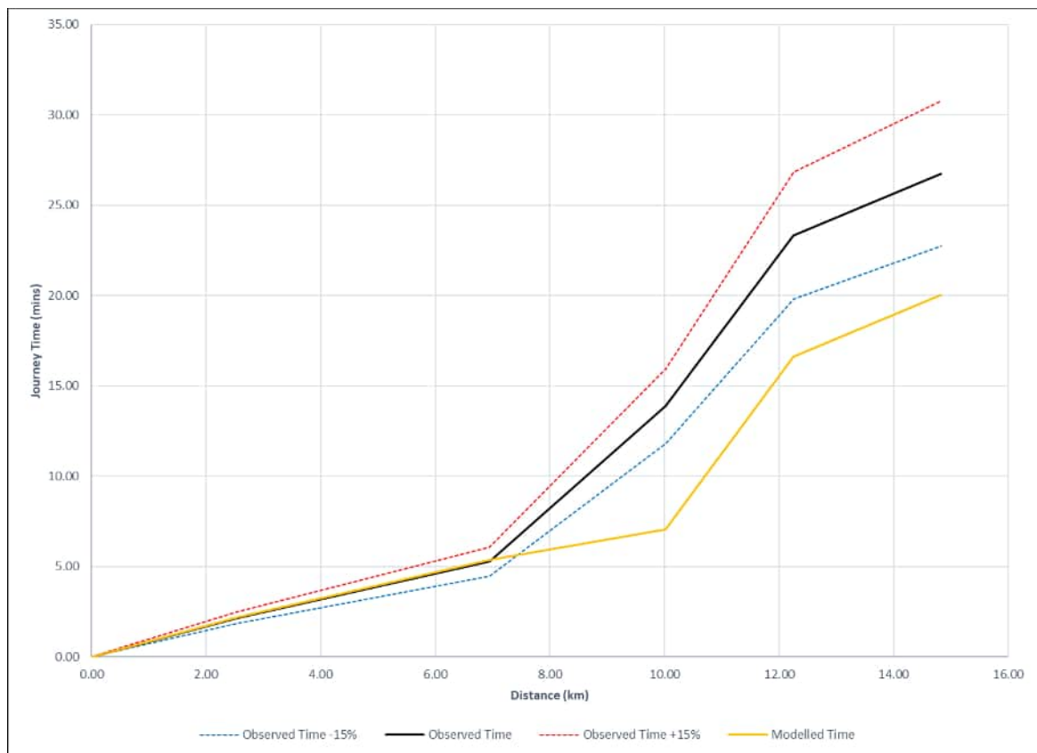
Plate E.62 Route 126 – A13 M25 junction – North Circular WB (AM peak HGV)
