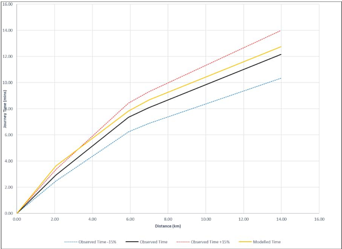
Plate E.94 Route 119 – A20 South Circular – M25 junction EB (inter-peak Lights)
