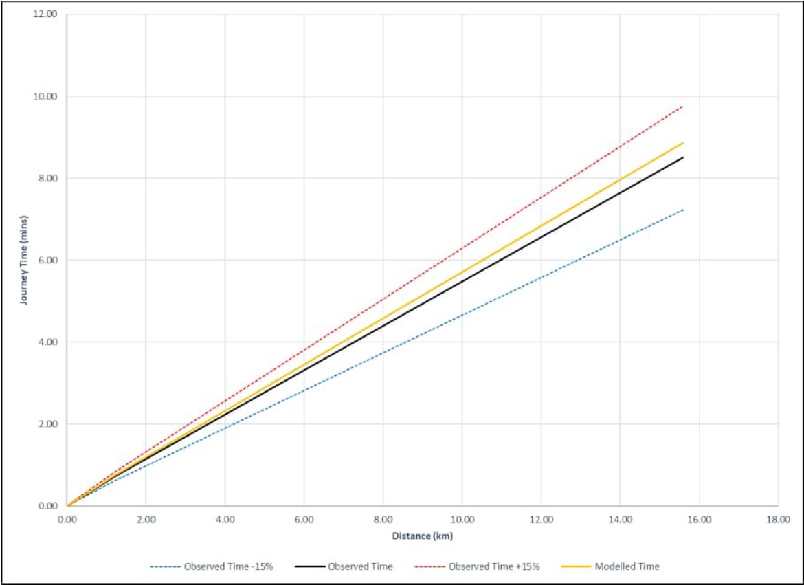
Plate E.111 Route 146 – M26 M20 junction – M25 junction WB (inter-peak Lights)
