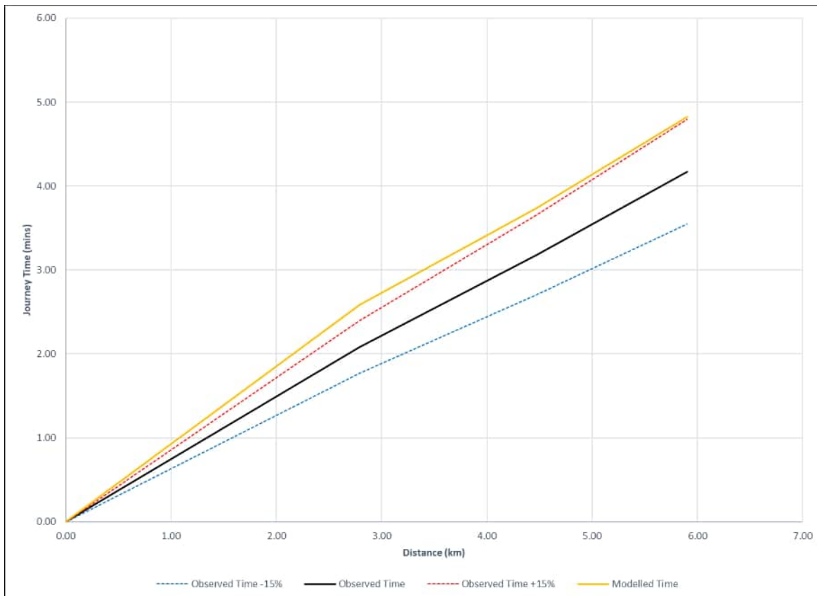
Plate E.193 Route 158 – A229 M2 junction – M20 junction SB (PM peak Lights)
