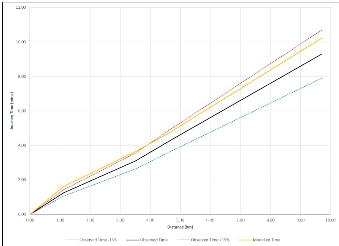
Plate E.34 Route 153 – A228 M20 junction – M2 junction NB (AM peak lights)
