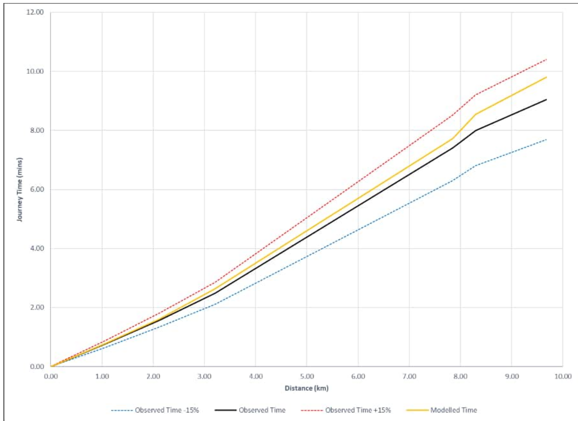
Plate E.43 Route 104W – M25 junction 2 – junction 30 ACW (A282) via west tunnel (AM peak HGV)
