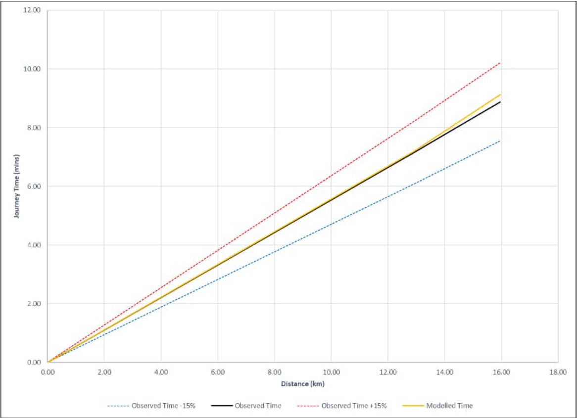
Plate E.110 Route 145 – M26 M25 junction – M20 junction EB (inter-peak Lights)
