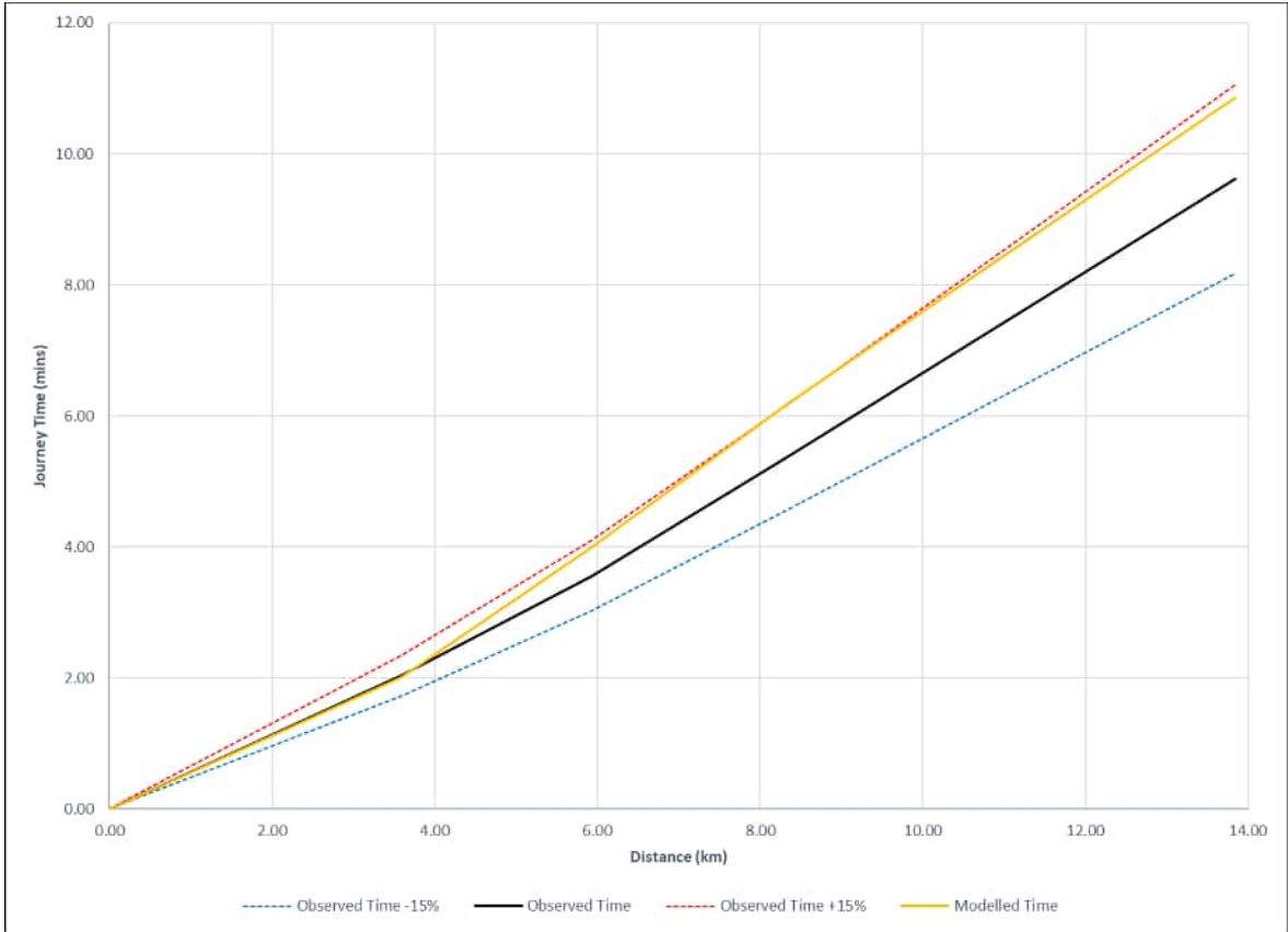
Plate E.87 Route 112 – A2 M25 junction – South Circular WB (inter-peak Lights)
