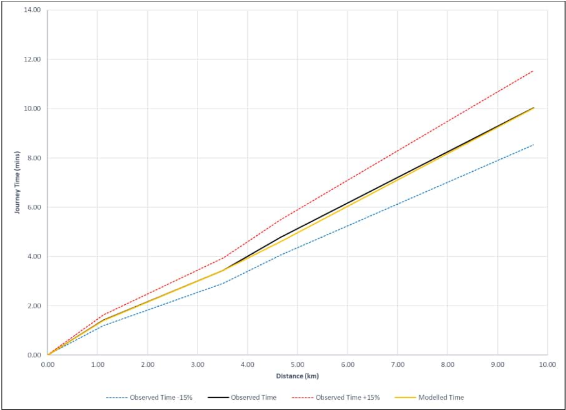
Plate E.152 Route 154 – A228 M2 junction – M20 junction SB (inter-peak HGV)
