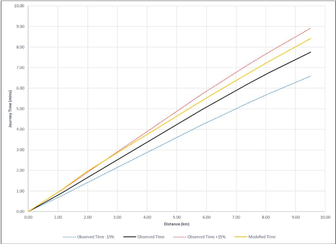
Plate E.42 Route 103 – M25 junction 30 – junction 2 CW (A282) (AM peak HGV)
