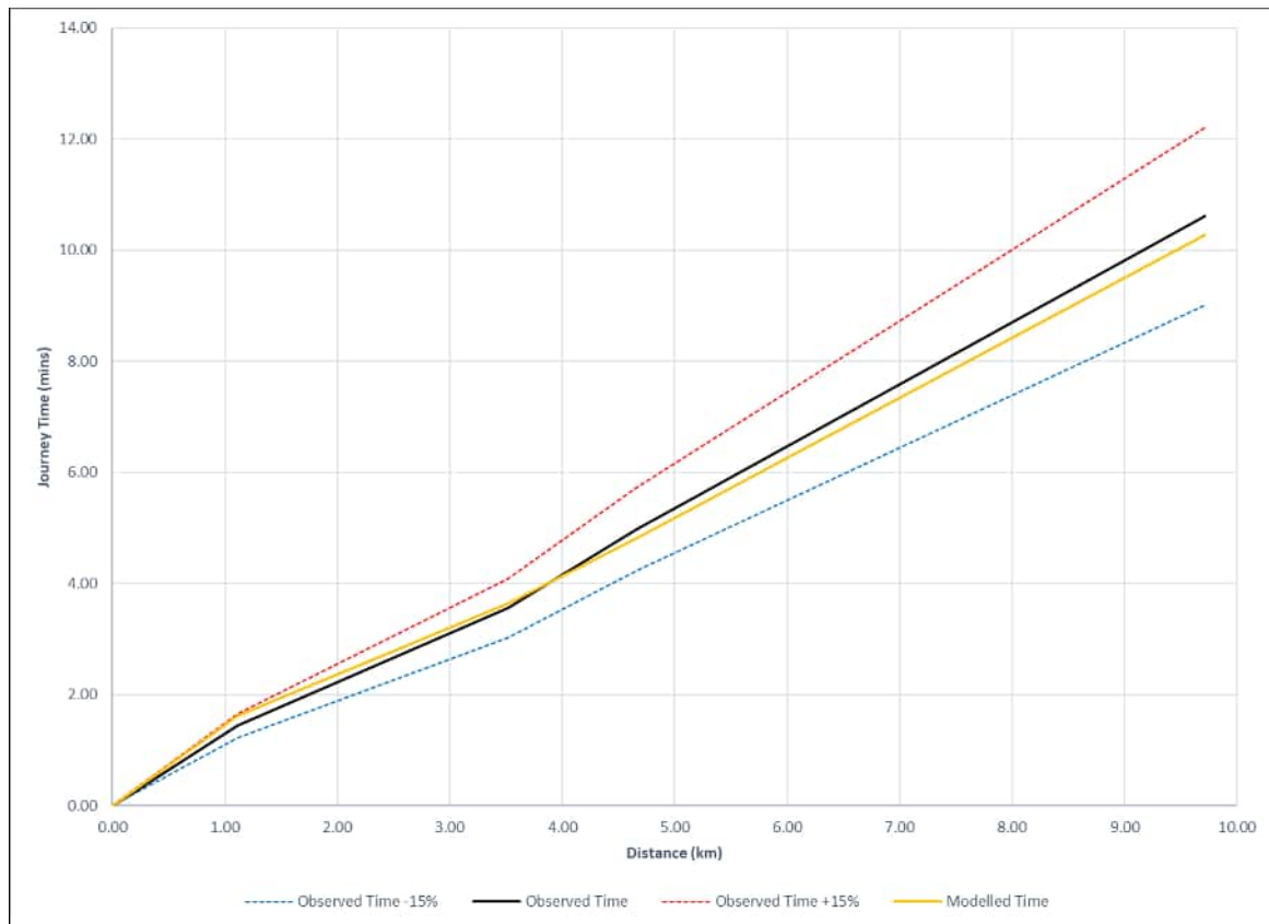
Plate E.73 Route 153 – A228 M20 junction – M2 junction NB (AM peak HGV)
