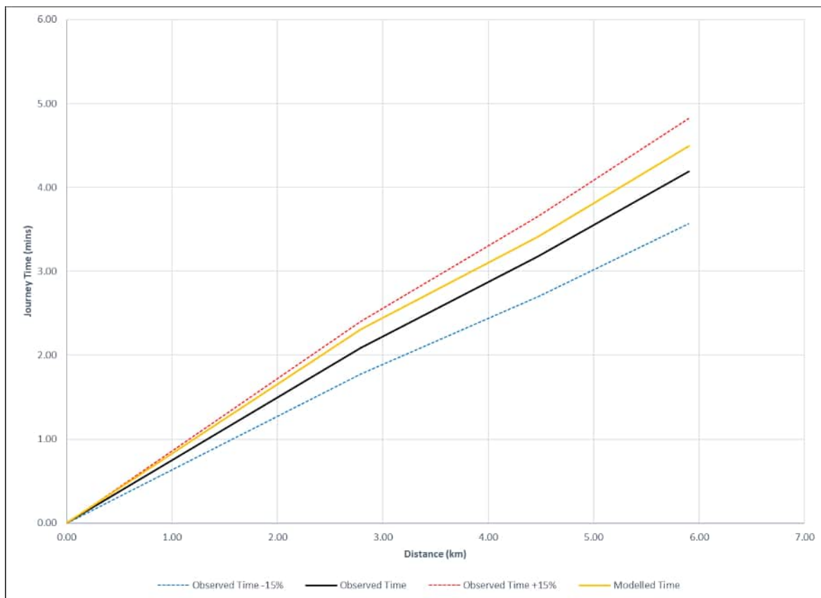
Plate E.115 Route 158 – A229 M2 junction – M20 junction SB (inter-peak Lights)
