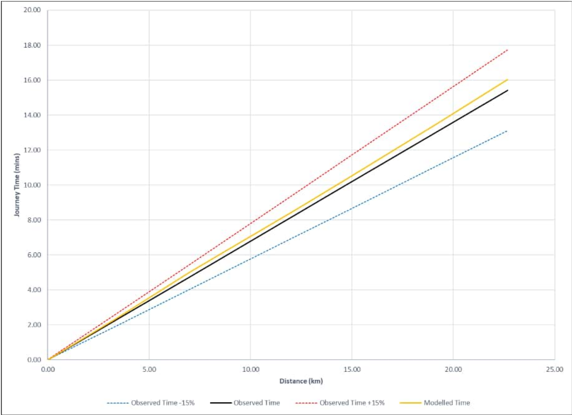
Plate E.146 Route 132 – A12 Chelmsford – M25 junction WB (inter-peak HGV)
