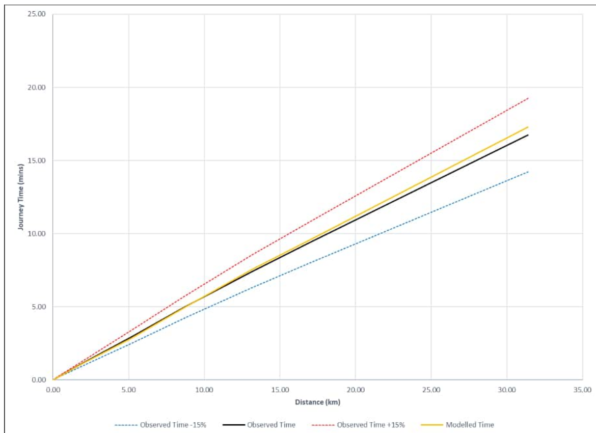
Plate E.175 Route 122 – M20 junction 7 – junction 1 WB (PM peak Lights)
